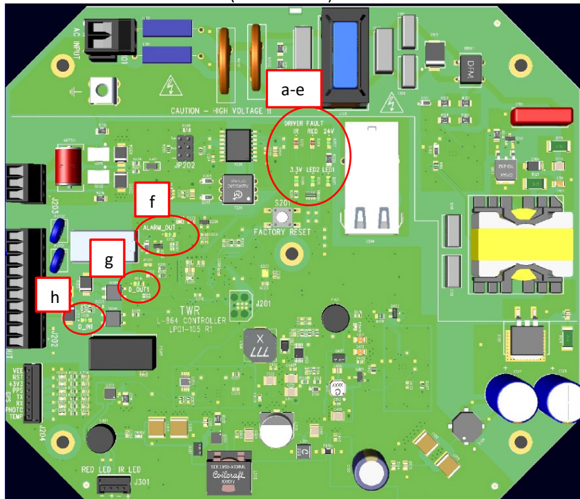
Figure 4 Power Supply LEDs
