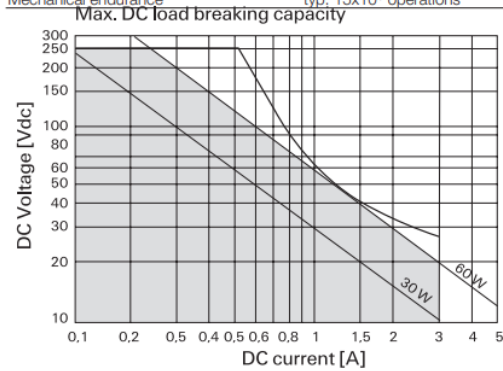
Figure 2 Alarm Relay Rating
