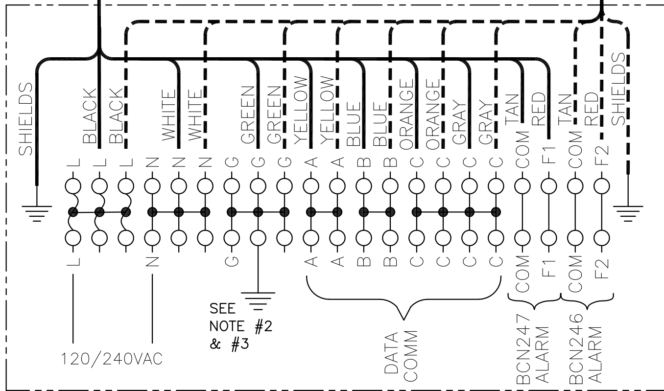
WIRING DIAGRAM
