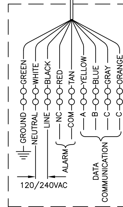
WIRING DIAGRAM
